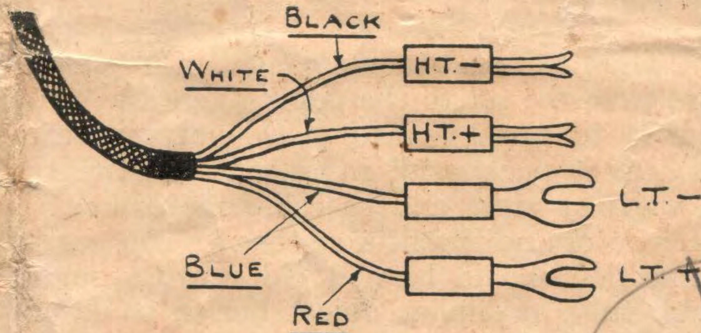
BATTERY CONNECTIONS.
